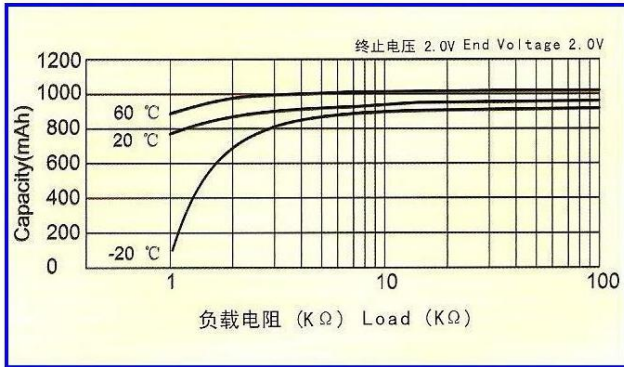
Load-capacity
